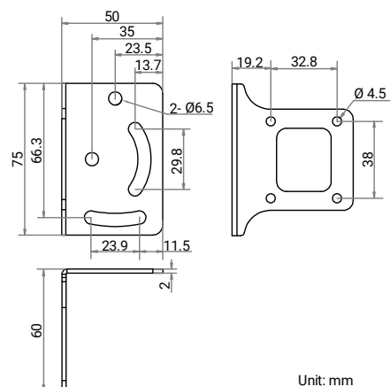
Installation Bracket:
